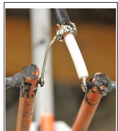
Figure 14: Feed point
